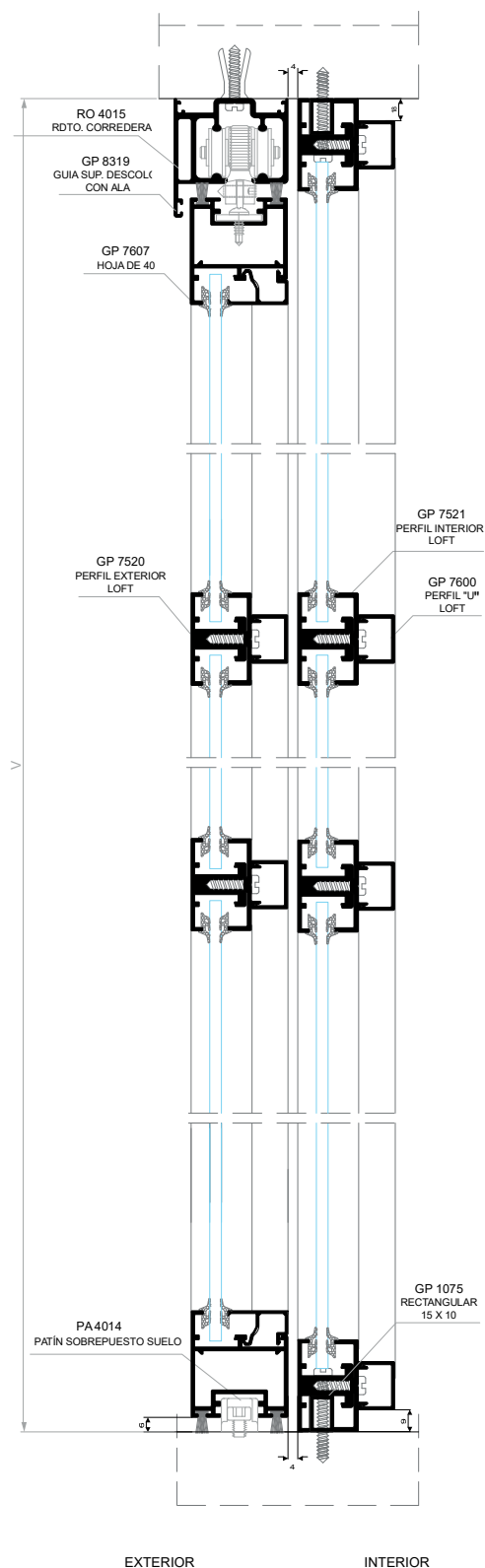
DETALLE CORREDERA + LOFT INDUSTRIAL
